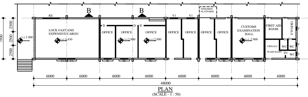
EXISTING ARRANGEMENTS OF GROUND FLOOR OF CFS OFFICE
