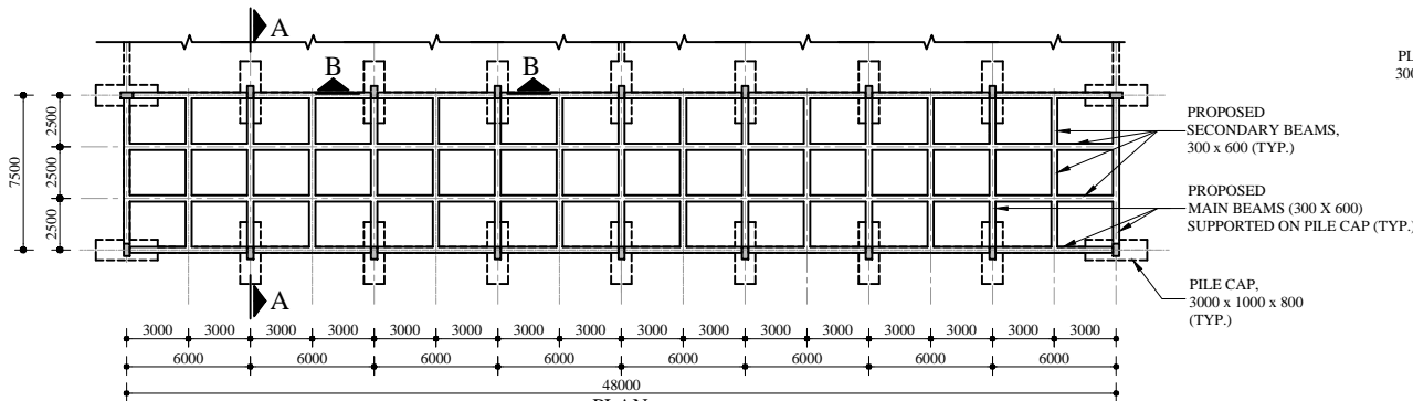
LAYOUT OF PROPOSED BEAMS AT GROUND FLOOR OF CFS
